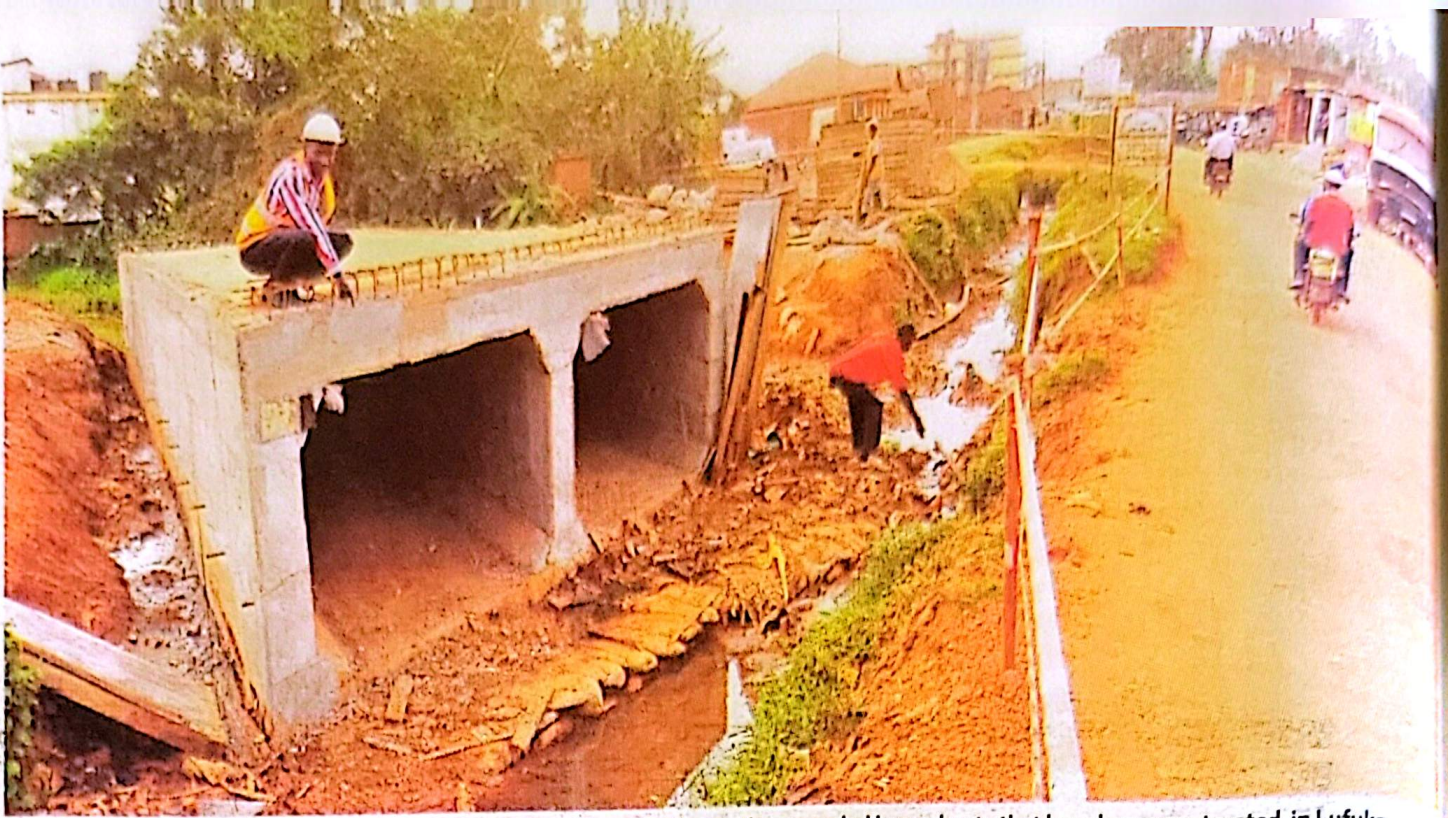
Improved. Abubaker Technical services engineer Godfrey Kyeyune shows the upgraded box culverts that have been constructed in Lufuka wetland on the Ndejje-Namasuba-Kitiko Road. PHOTO BY JOSEPH KIGGUNDU
